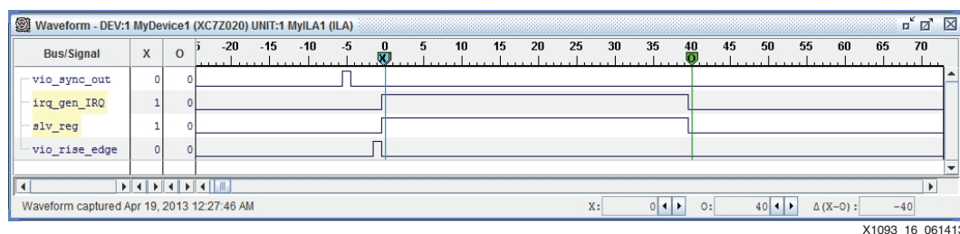
Figure 16: Chipscope Subsequent Capture
