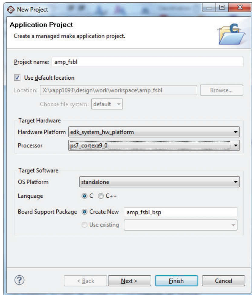
Figure 3: Create FSBL
